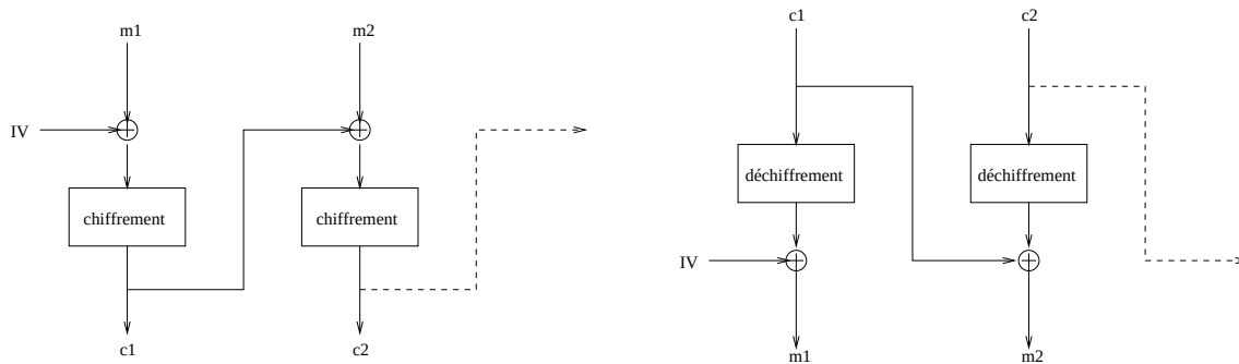
Figure 9. Le mode CBC
