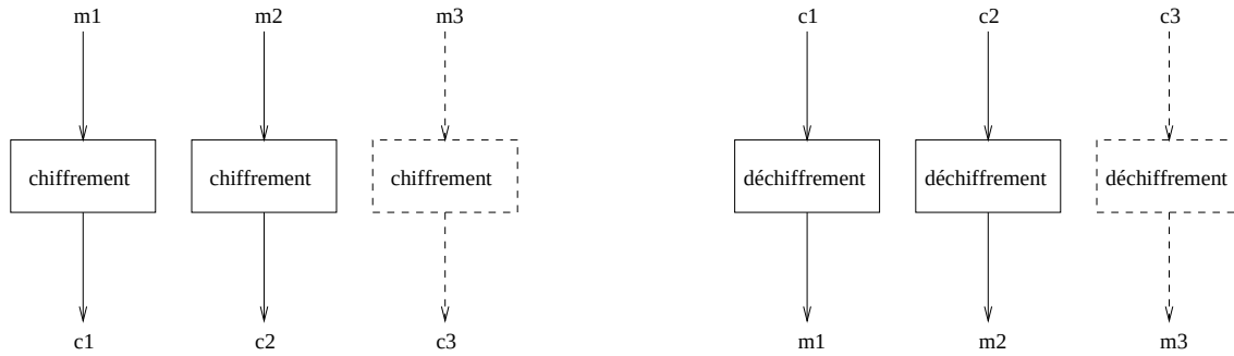
Figure 8. Le mode ECB
