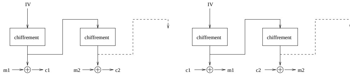
Figure 10. Le mode OFB
