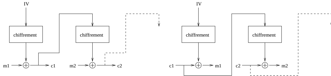
Figure 11. Le mode CFB
