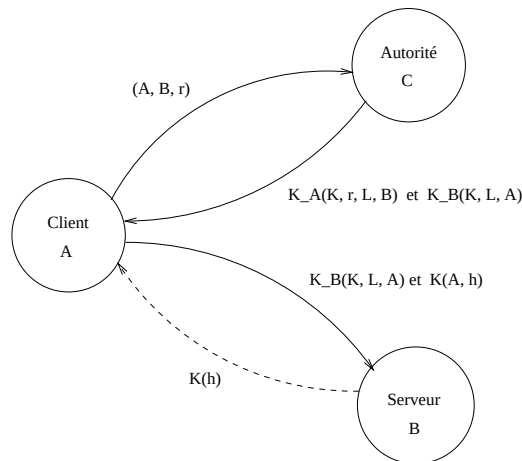
Figure 9. Protocole Kerberos
