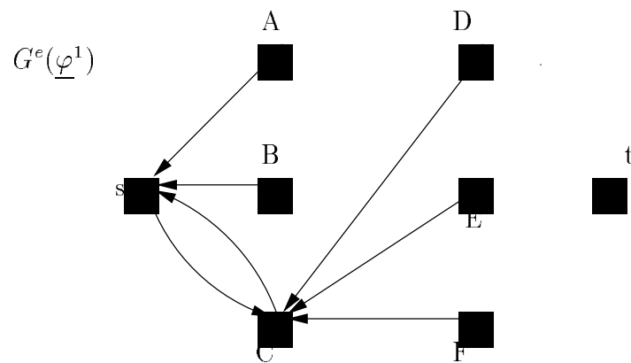
FIG. 4.5 - Flot maximum
