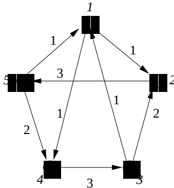
FIG. 4.1 – Flot initial
